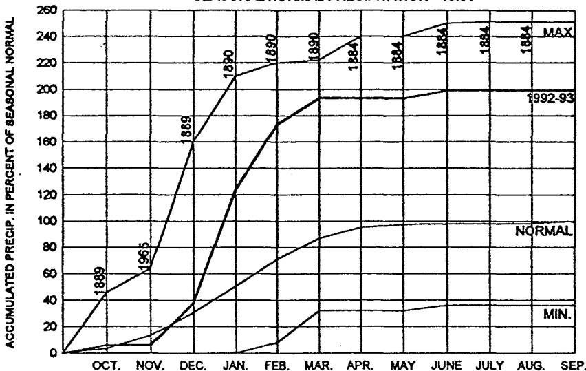
LOS ANGELES (STATION #716) SEASONAL NORMAL PRECIPITATION - 15.51"
